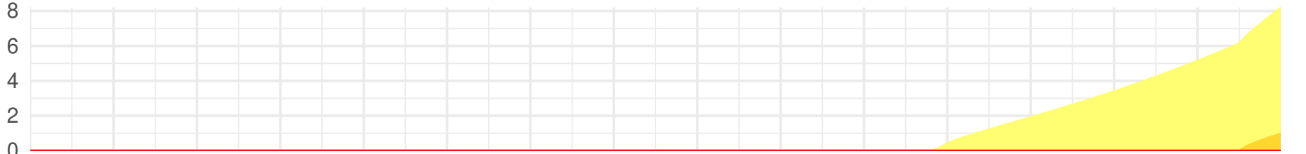
Accelerating Emissions (SSP5-8.5)
